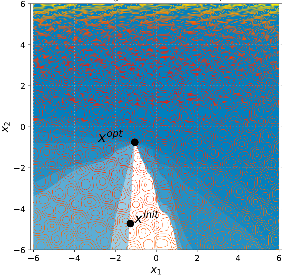
54 Rotated Rastrigin with 6+3n constraints, instance=9
