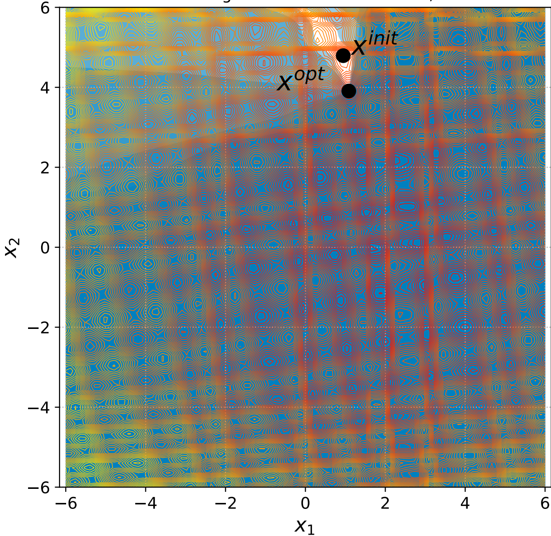
54 Rotated Rastrigin with 6+3n constraints, instance=8
