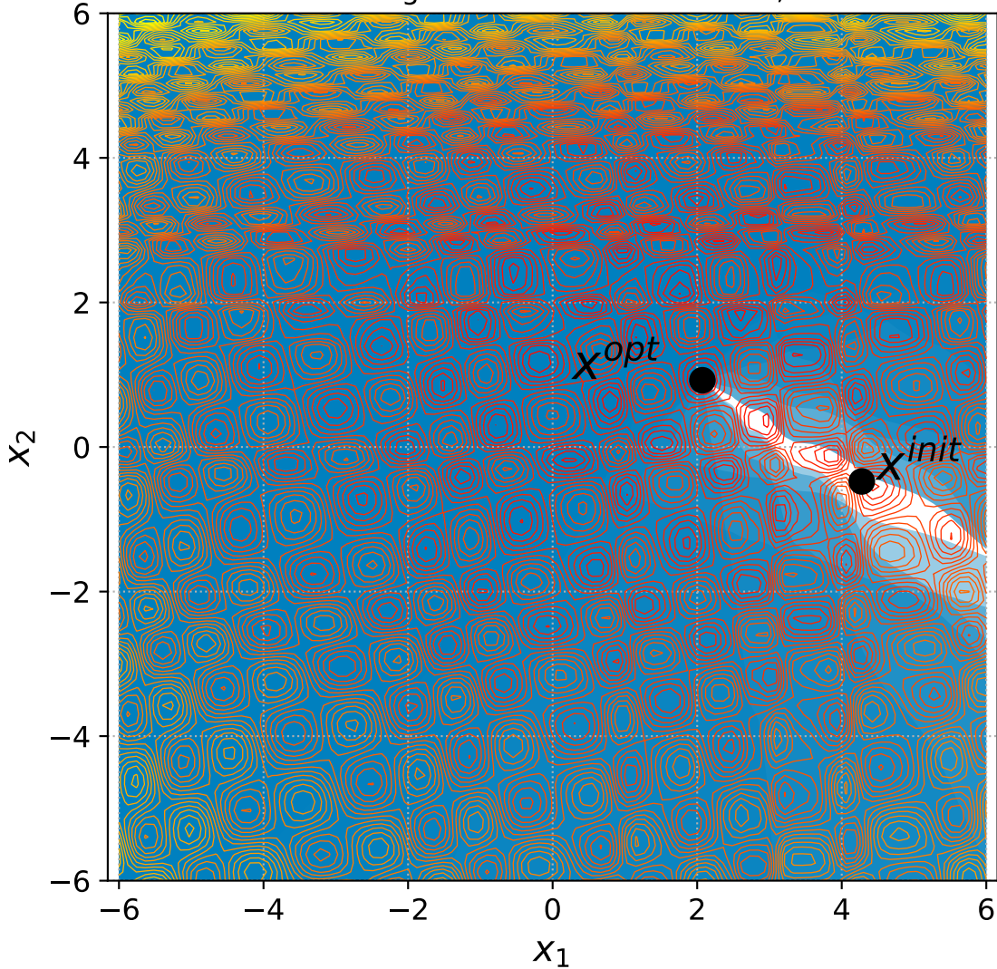
54 Rotated Rastrigin with 6+3n constraints, instance=6
