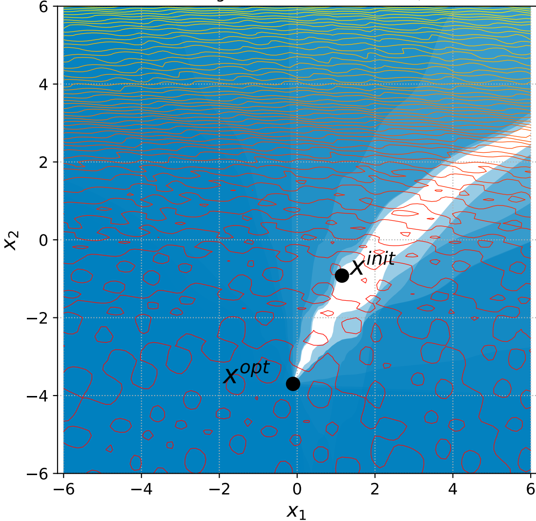
54 Rotated Rastrigin with 6+3n constraints, instance=5
