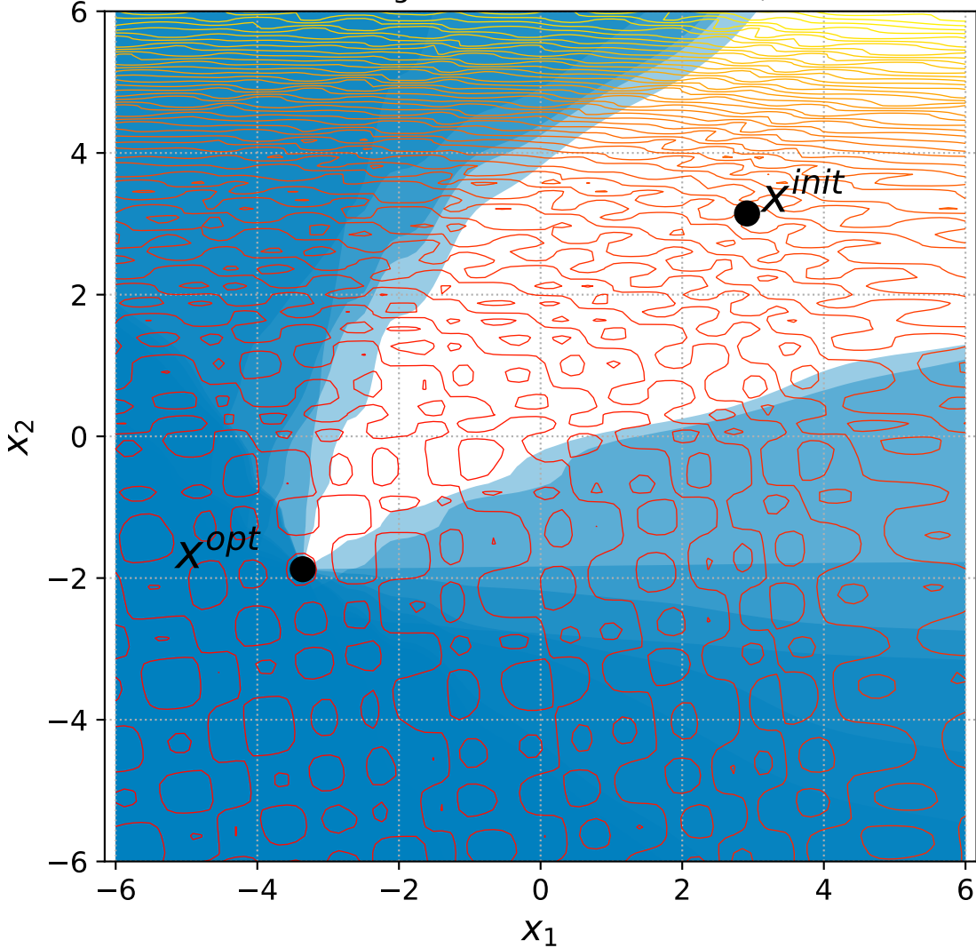
54 Rotated Rastrigin with 6+3n constraints, instance=4
