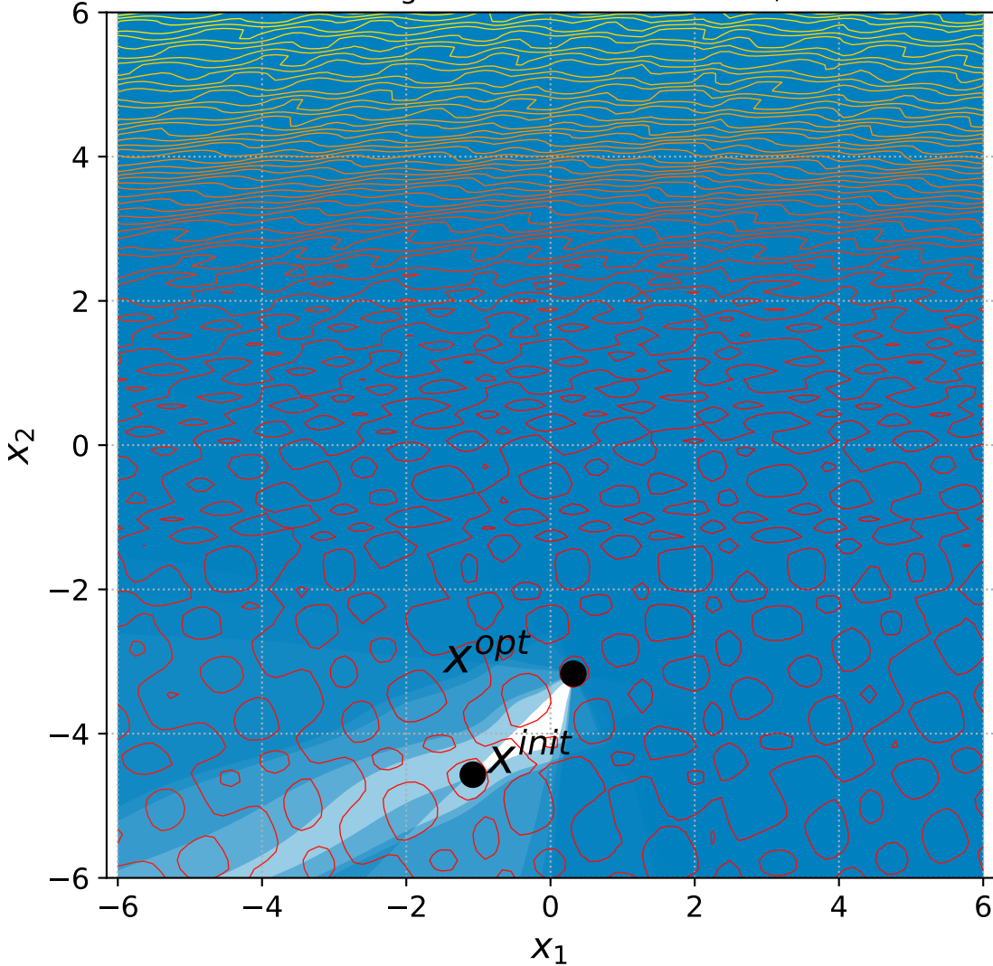
54 Rotated Rastrigin with 6+3n constraints, instance=3
