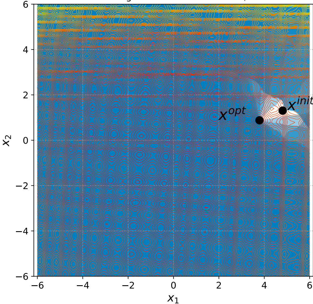
54 Rotated Rastrigin with 6+3n constraints, instance=2
