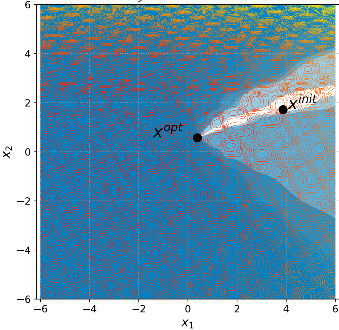
54 Rotated Rastrigin with 6+3n constraints, instance=1
