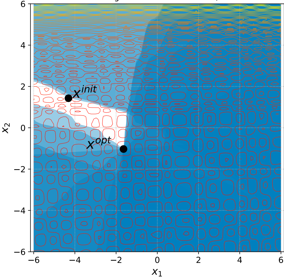
53 Rotated Rastrigin with 6+n constraints, instance=15
