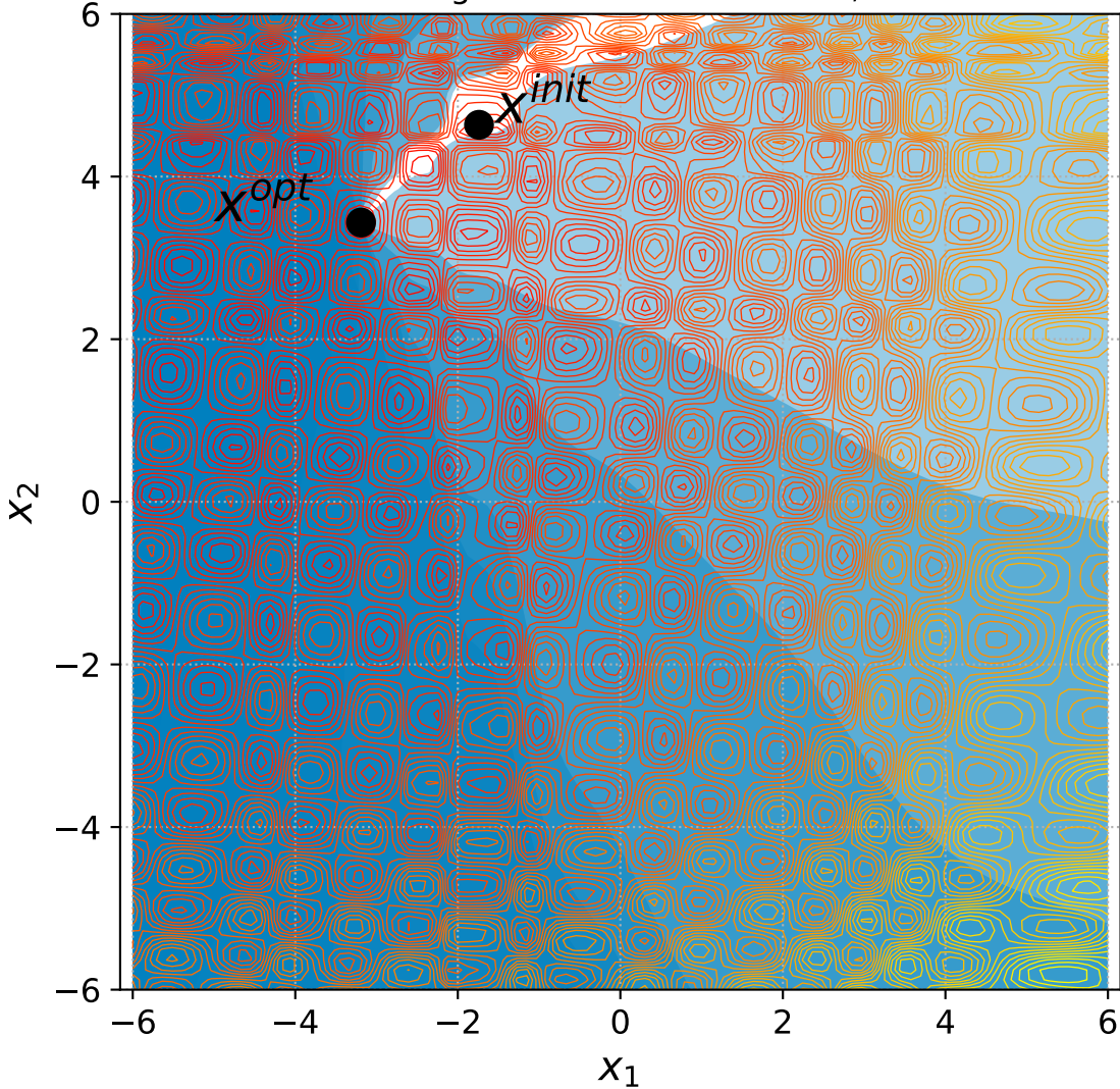
53 Rotated Rastrigin with 6+n constraints, instance=14
