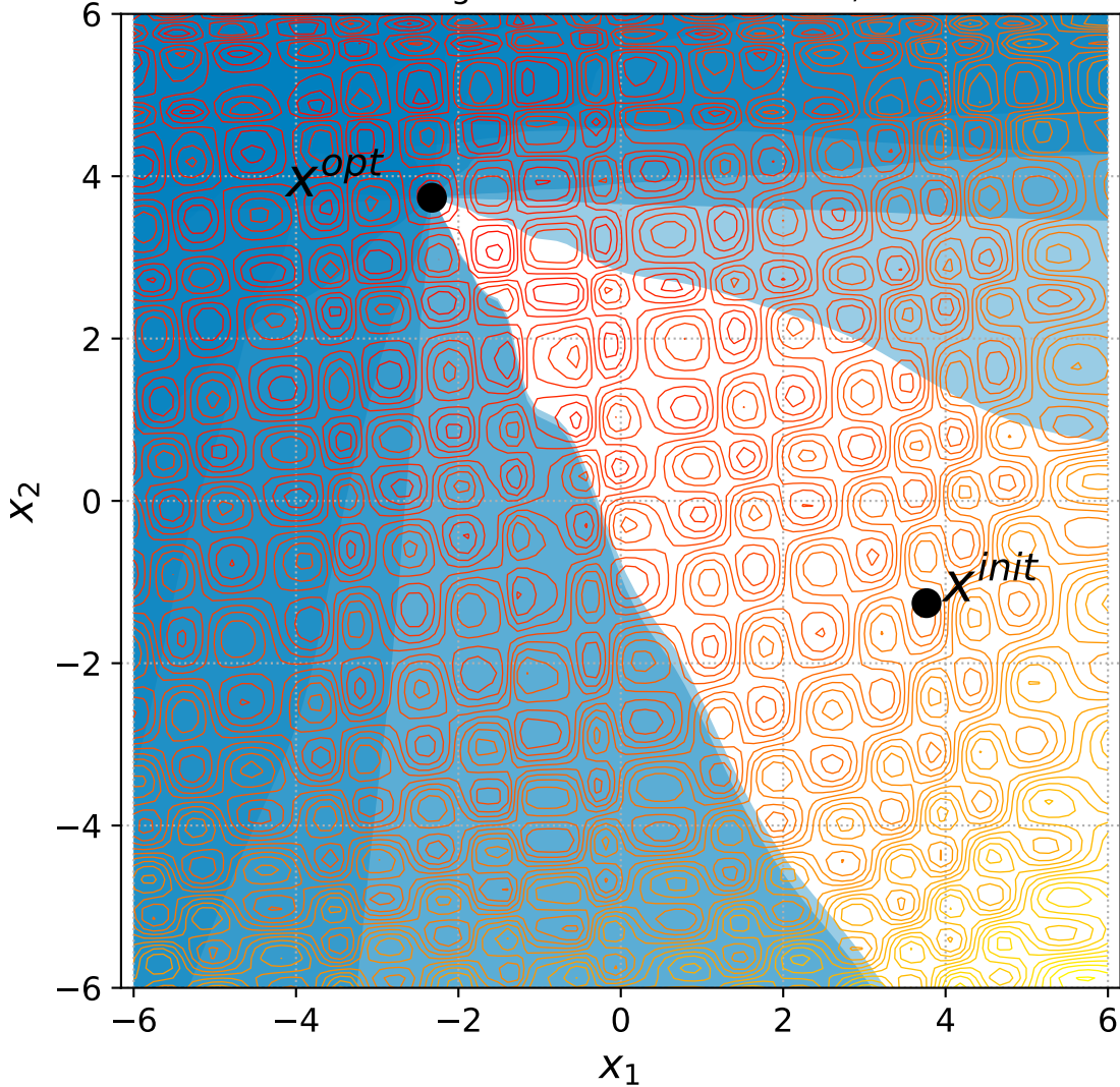
53 Rotated Rastrigin with 6+n constraints, instance=10
