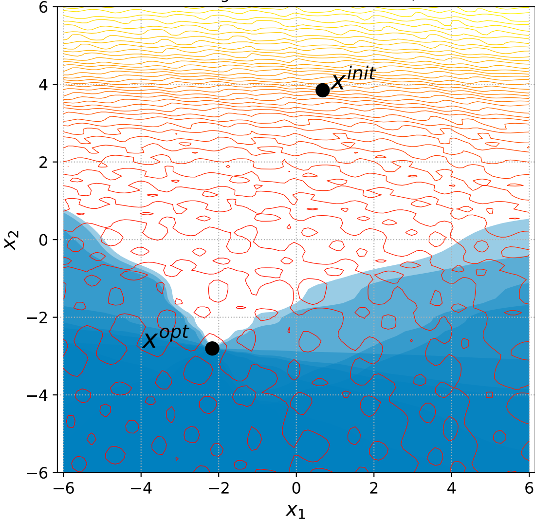
53 Rotated Rastrigin with 6+n constraints, instance=8
