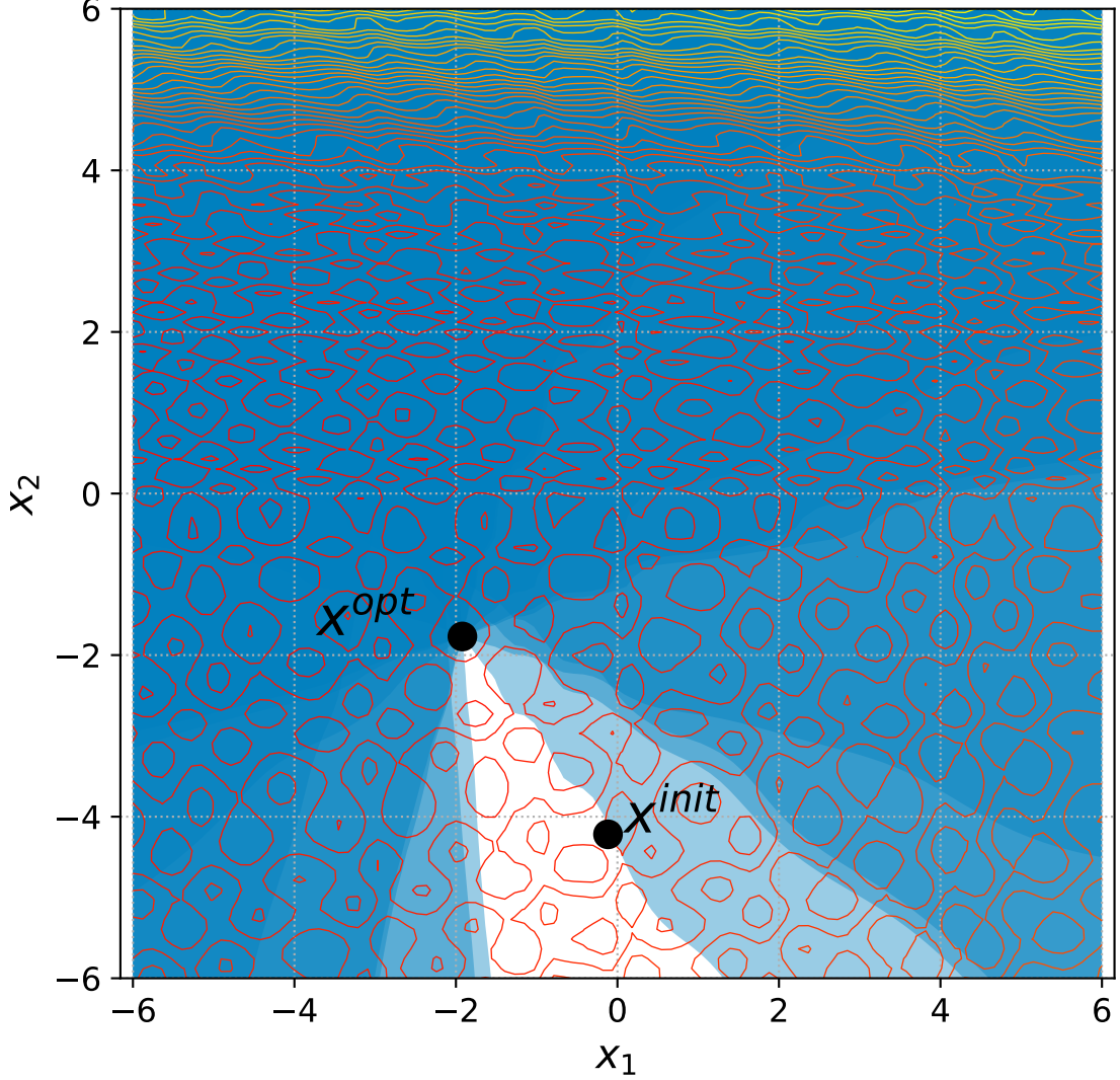
53 Rotated Rastrigin with 6+n constraints, instance=6
