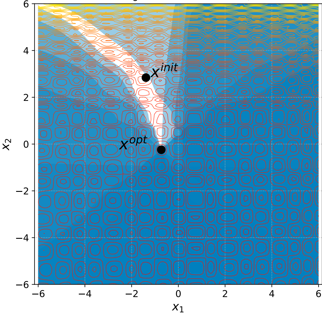
53 Rotated Rastrigin with 6+n constraints, instance=4
