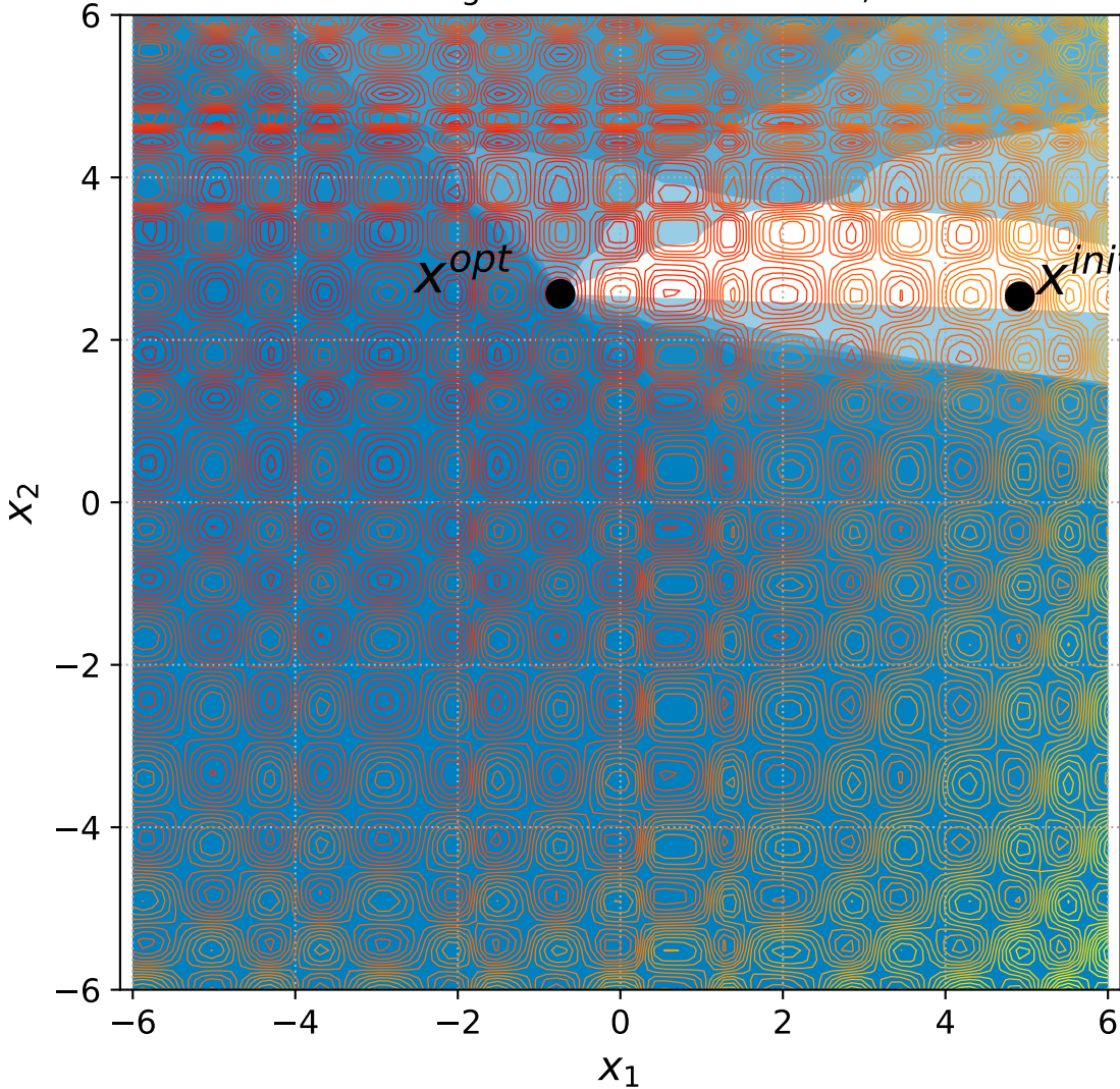
53 Rotated Rastrigin with 6+n constraints, instance=3
