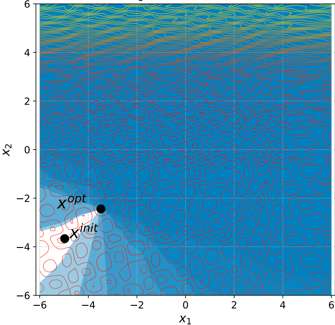
53 Rotated Rastrigin with 6+n constraints, instance=1
