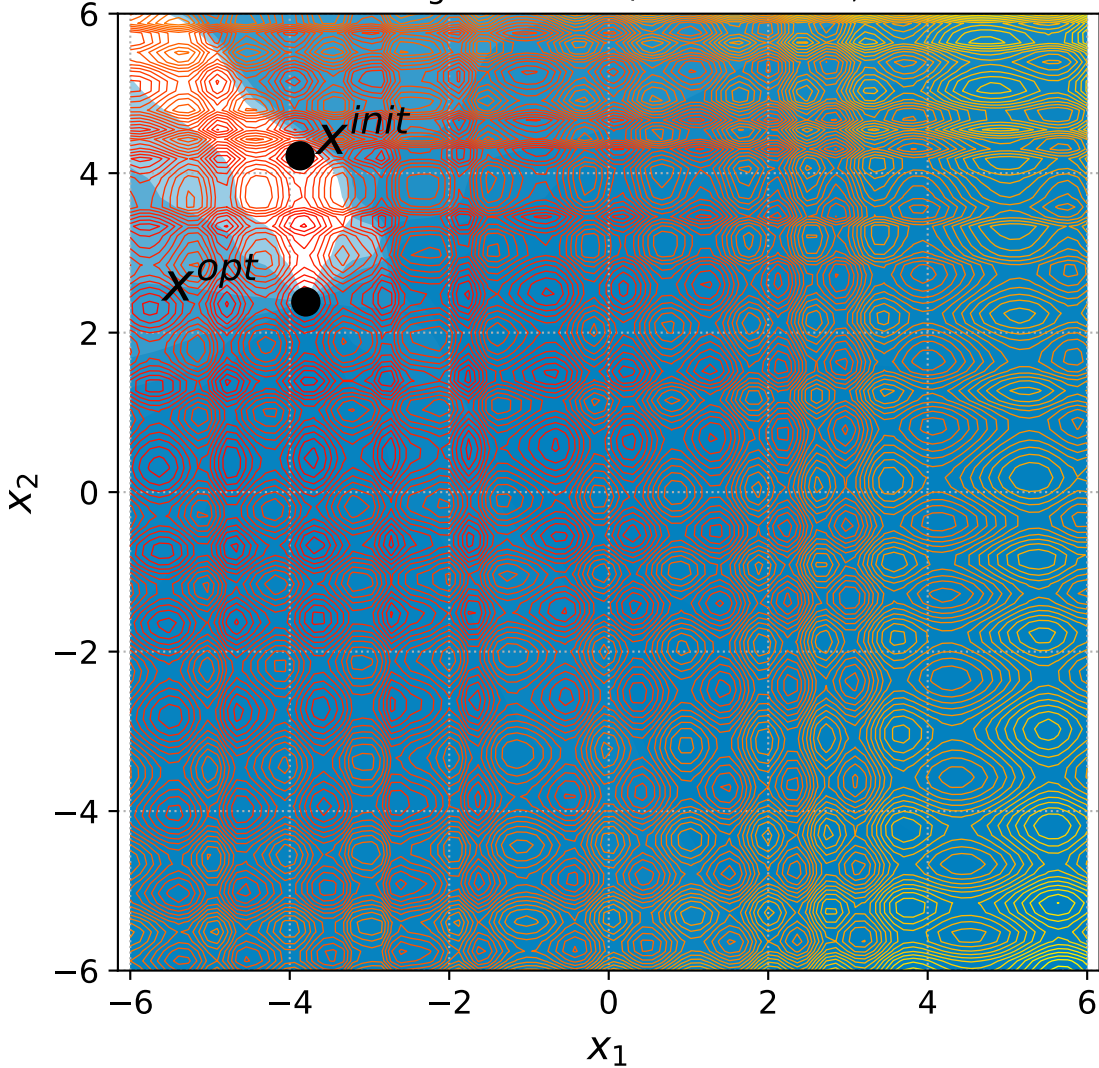
52 Rotated Rastrigin with 6+n/2 constraints, instance=15
