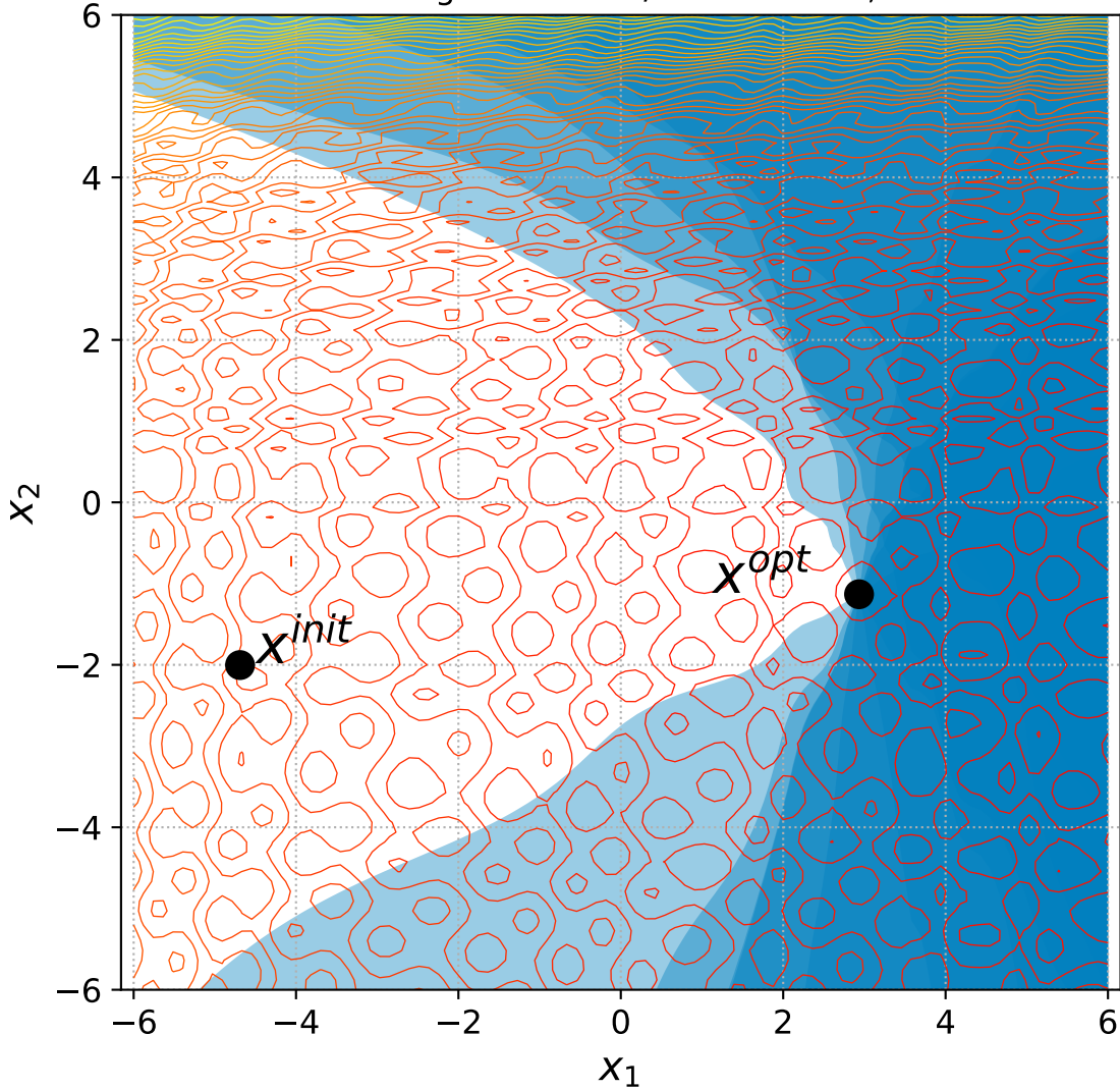
52 Rotated Rastrigin with 6+n/2 constraints, instance=14
