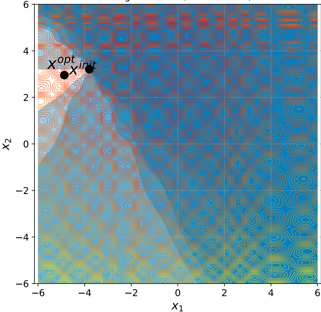
52 Rotated Rastrigin with 6+n/2 constraints, instance=13
