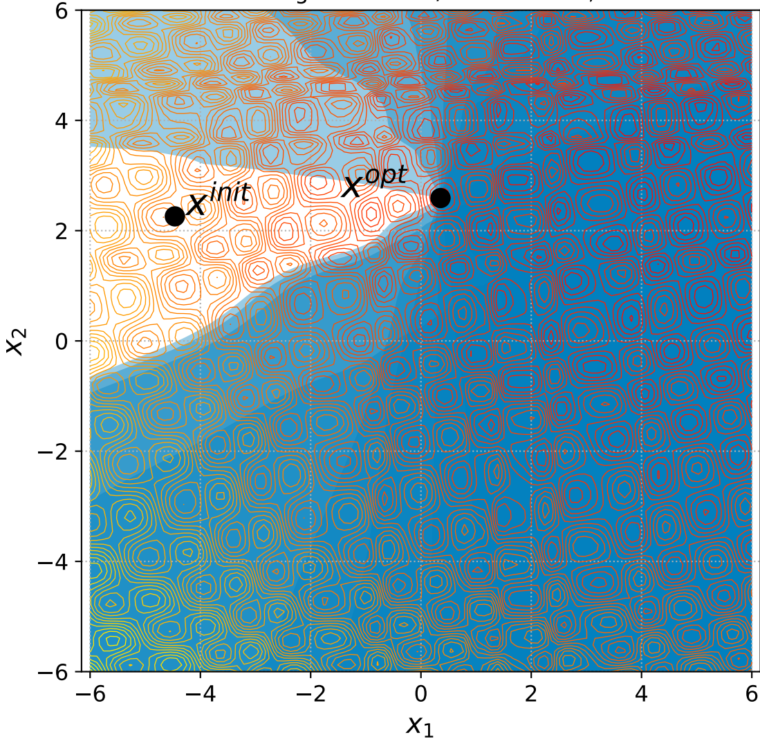
52 Rotated Rastrigin with 6+n/2 constraints, instance=12
