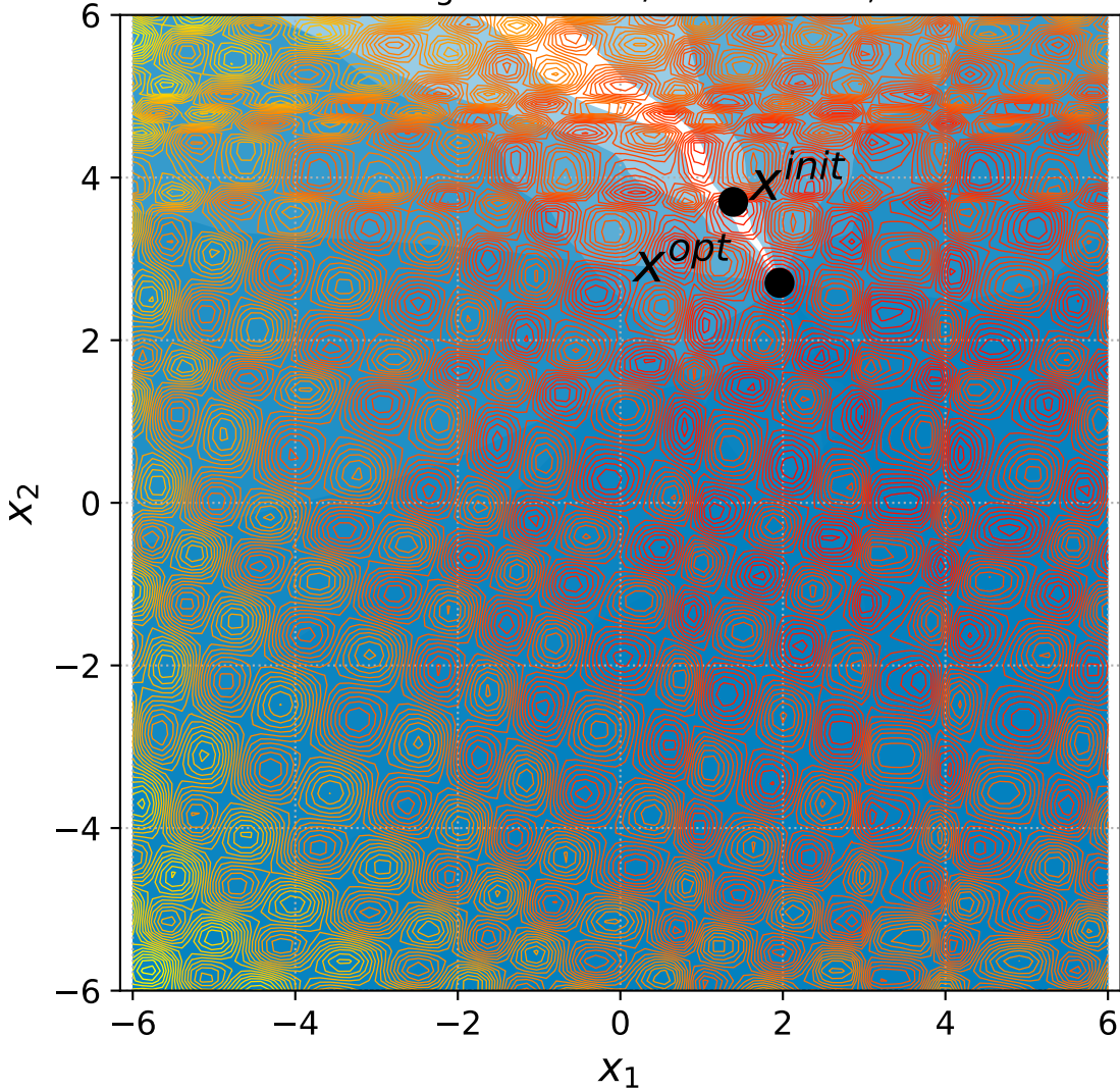
52 Rotated Rastrigin with 6+n/2 constraints, instance=10
