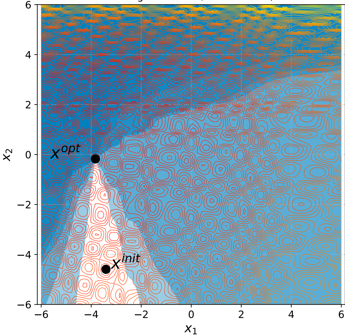
52 Rotated Rastrigin with 6+n/2 constraints, instance=9
