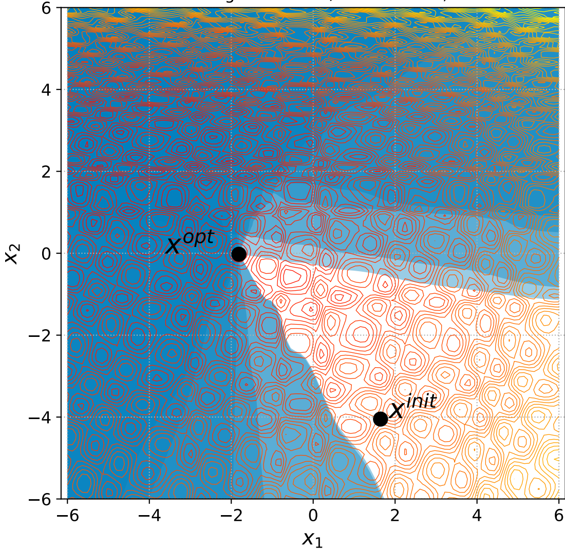
52 Rotated Rastrigin with 6+n/2 constraints, instance=7
