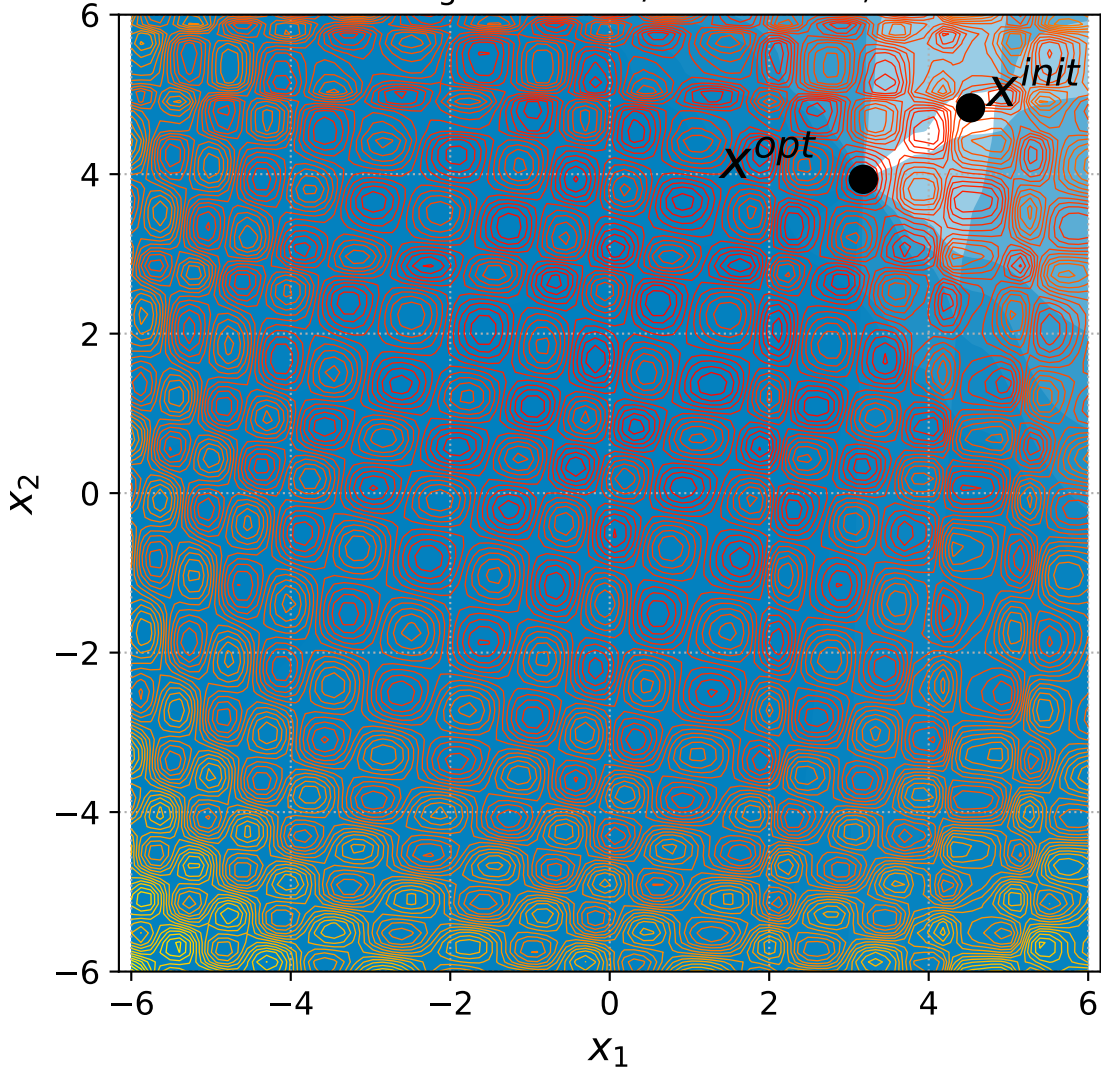
52 Rotated Rastrigin with 6+n/2 constraints, instance=6
