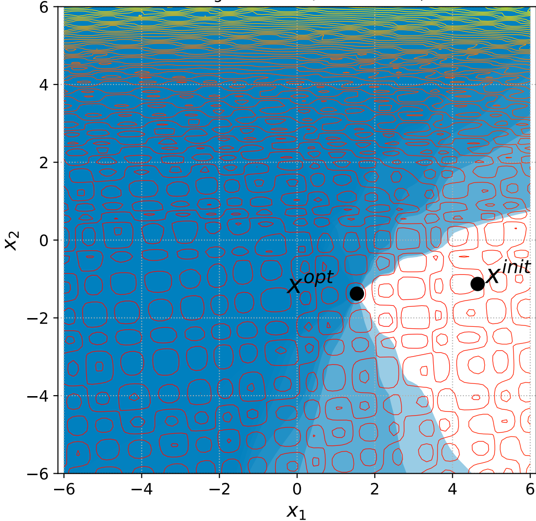
52 Rotated Rastrigin with 6+n/2 constraints, instance=4
