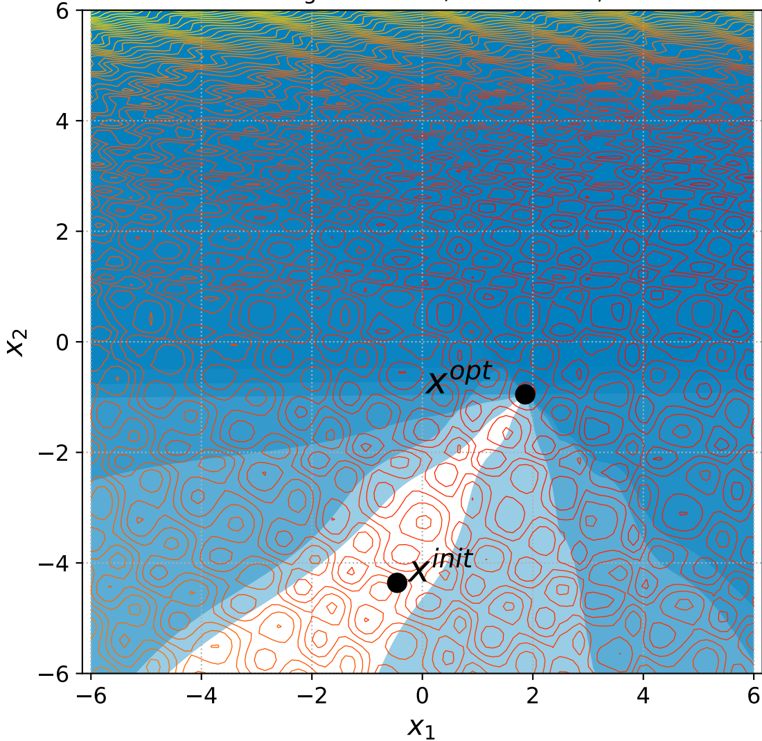
52 Rotated Rastrigin with 6+n/2 constraints, instance=3
