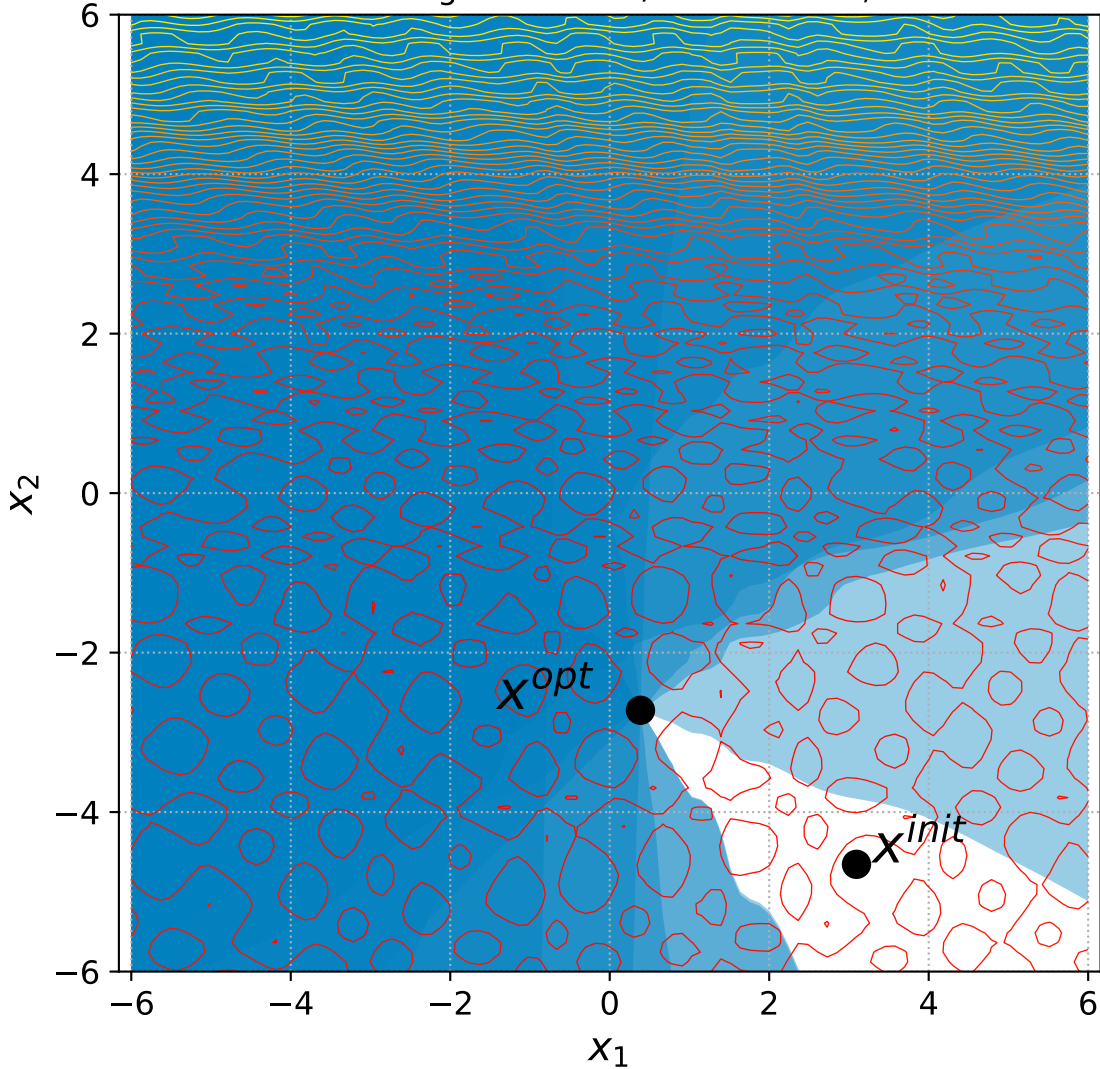
52 Rotated Rastrigin with 6+n/2 constraints, instance=2
