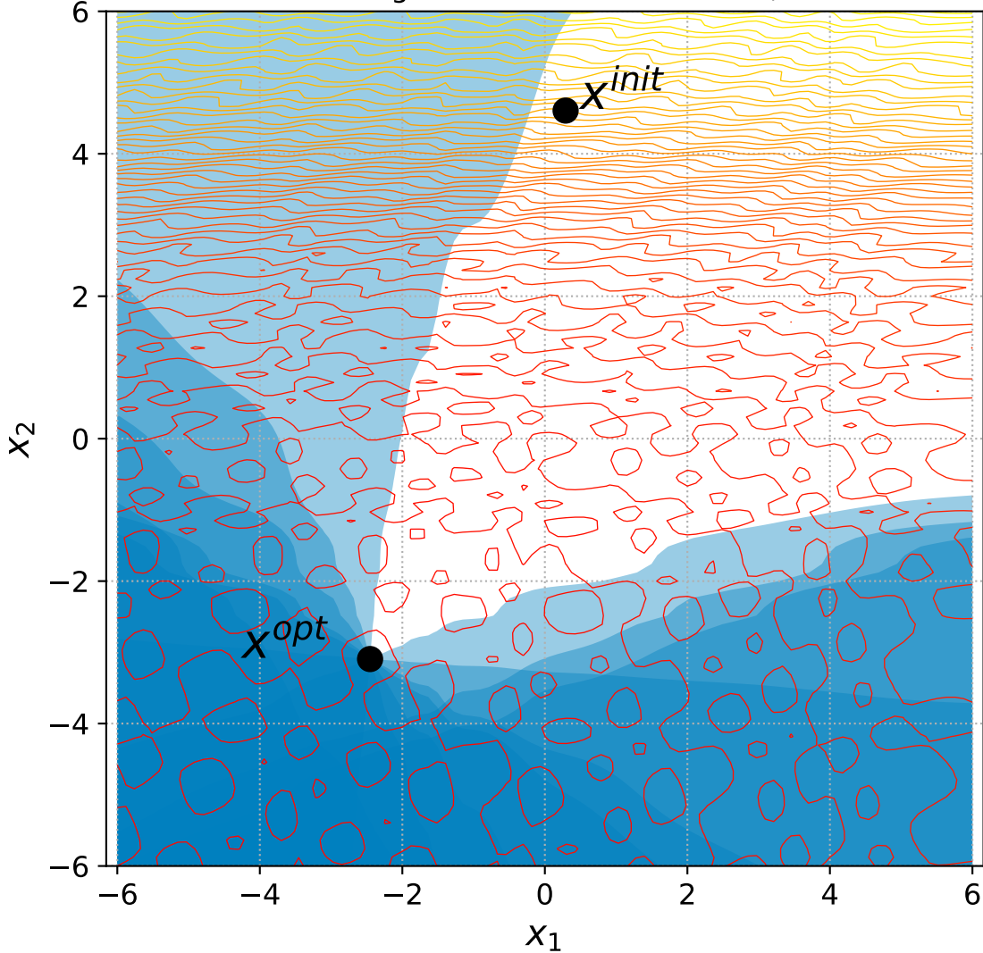
52 Rotated Rastrigin with 6+n/2 constraints, instance=1
