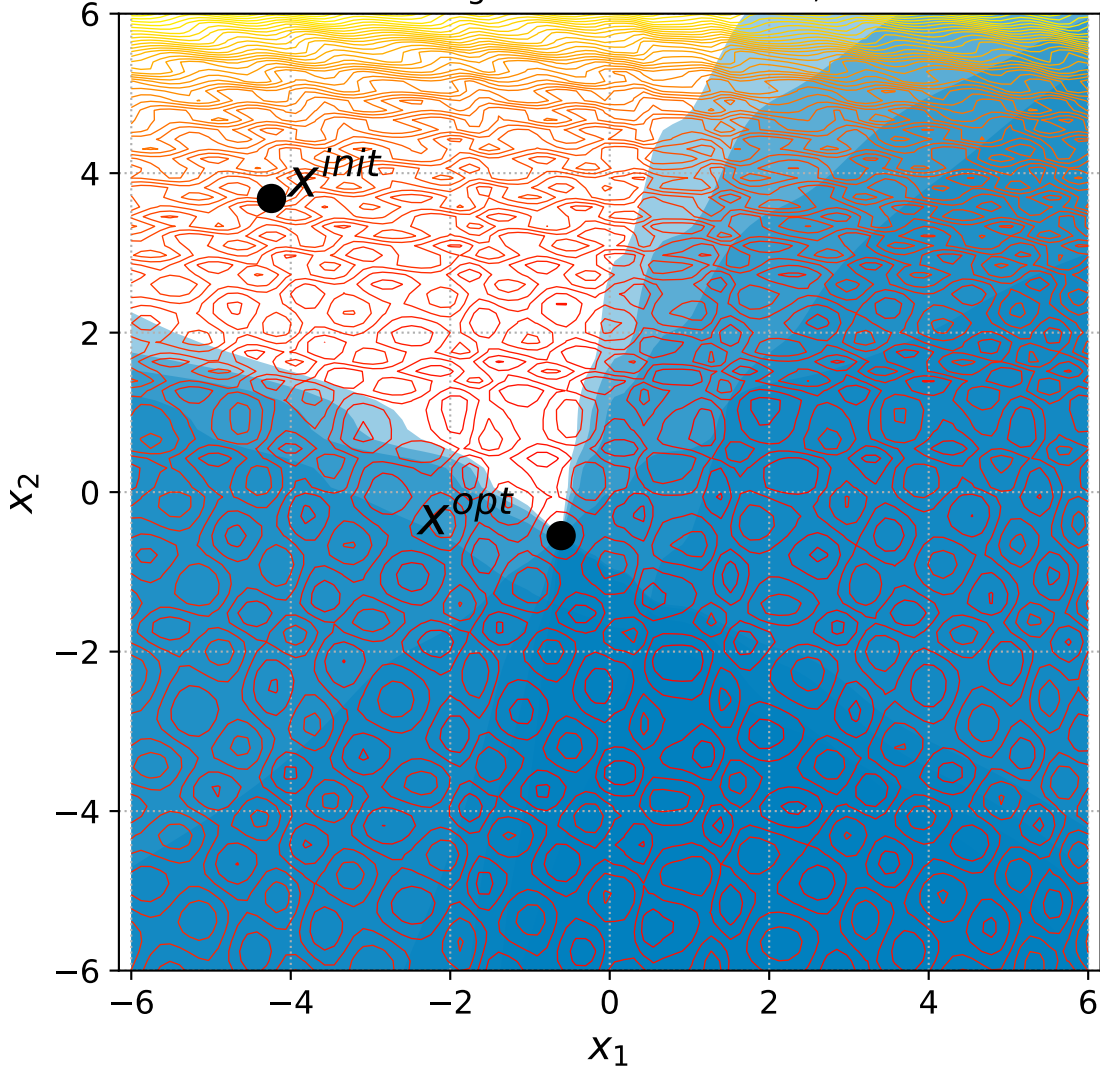
51 Rotated Rastrigin with 6 constraints, instance=15
