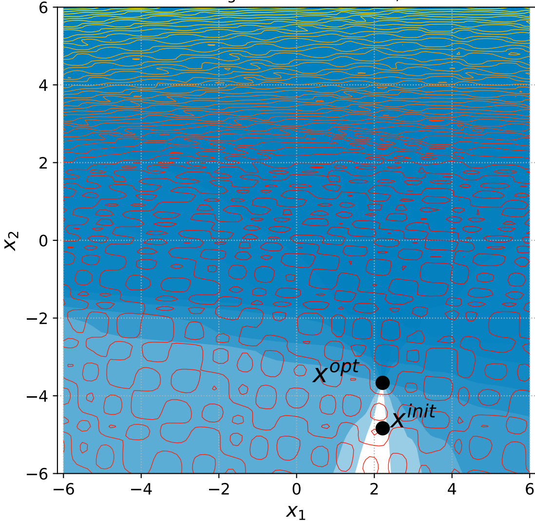
51 Rotated Rastrigin with 6 constraints, instance=14
