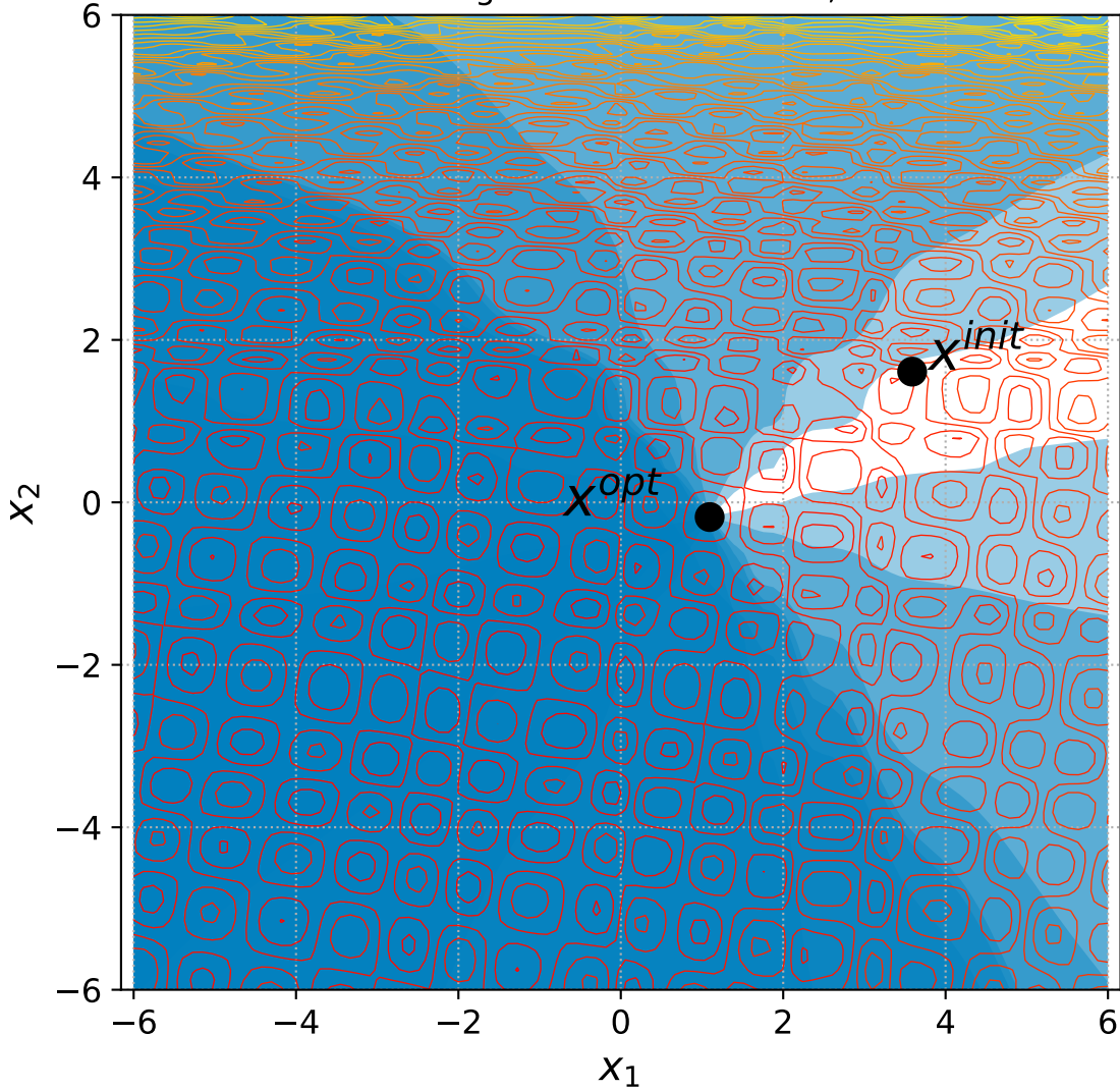
51 Rotated Rastrigin with 6 constraints, instance=12
