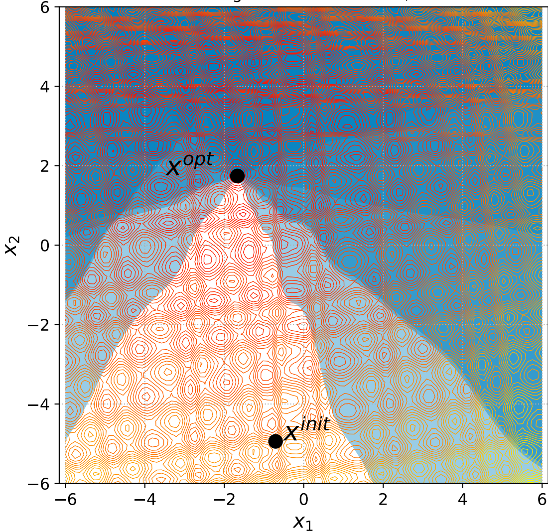
51 Rotated Rastrigin with 6 constraints, instance=11
