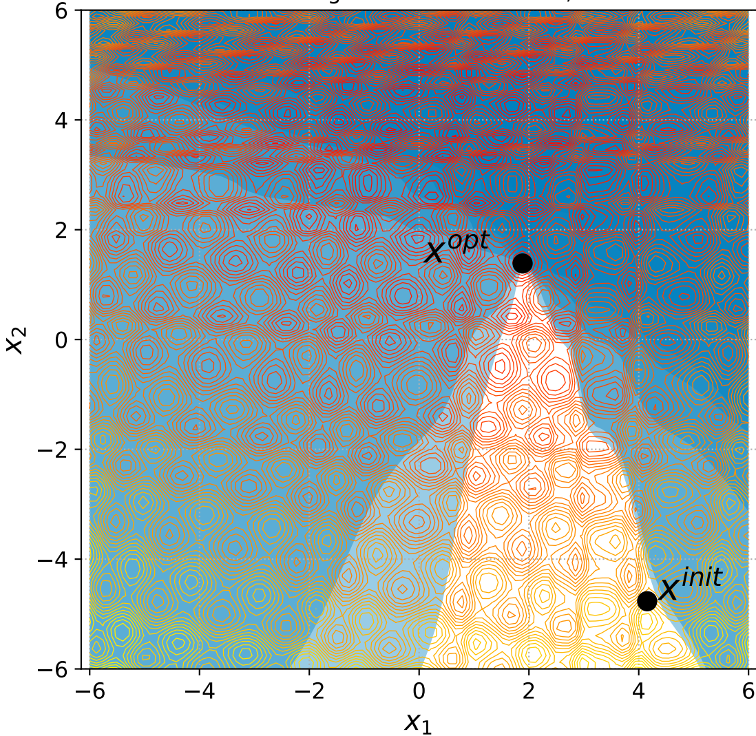
51 Rotated Rastrigin with 6 constraints, instance=9
