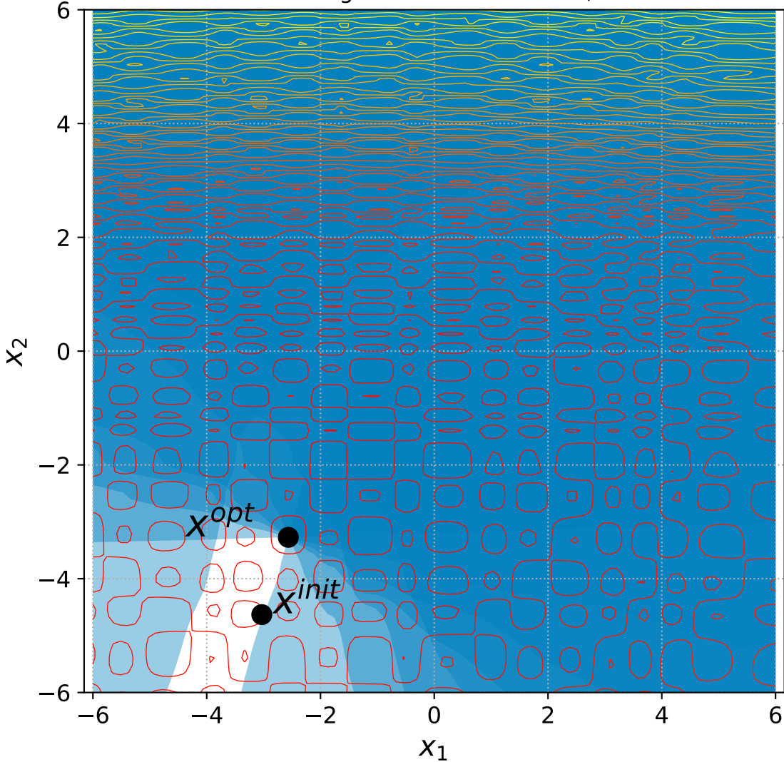
51 Rotated Rastrigin with 6 constraints, instance=8
