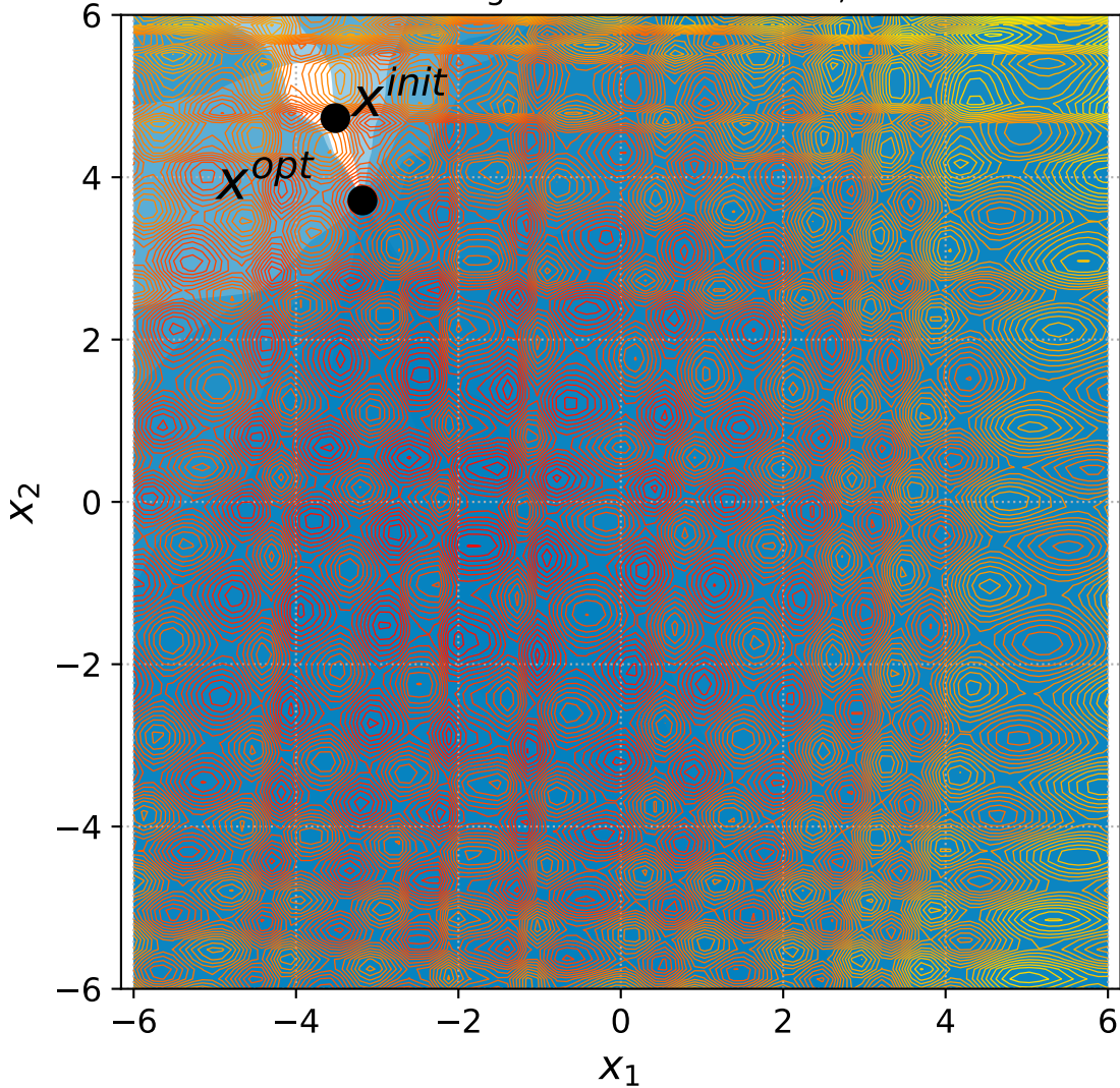
51 Rotated Rastrigin with 6 constraints, instance=7
