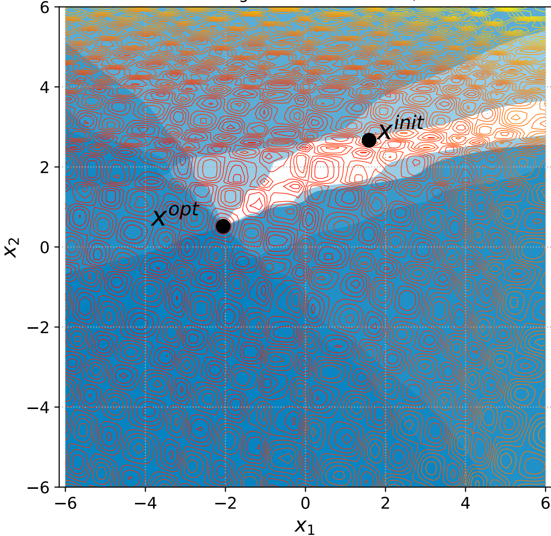
51 Rotated Rastrigin with 6 constraints, instance=6
