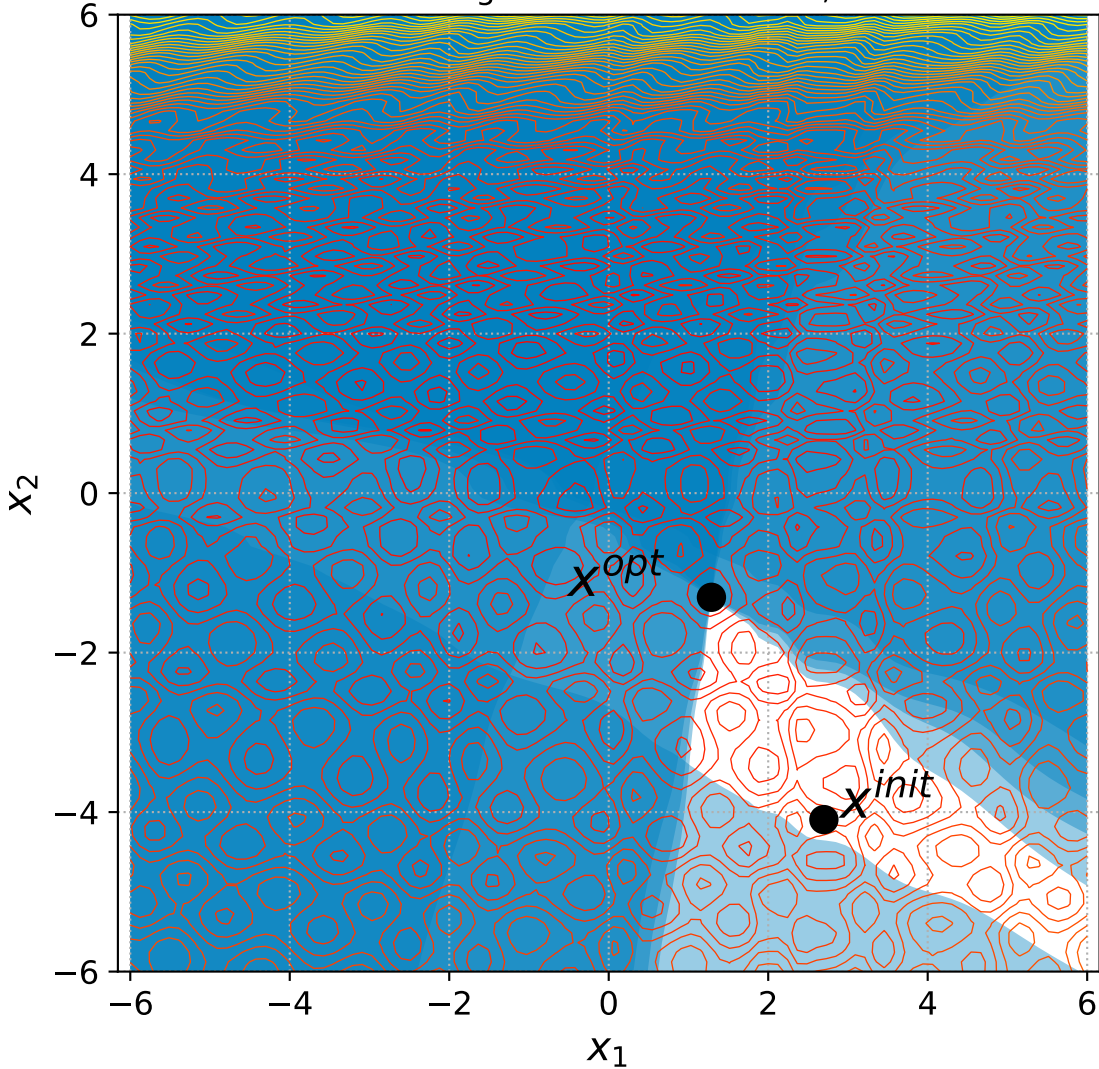
51 Rotated Rastrigin with 6 constraints, instance=5
