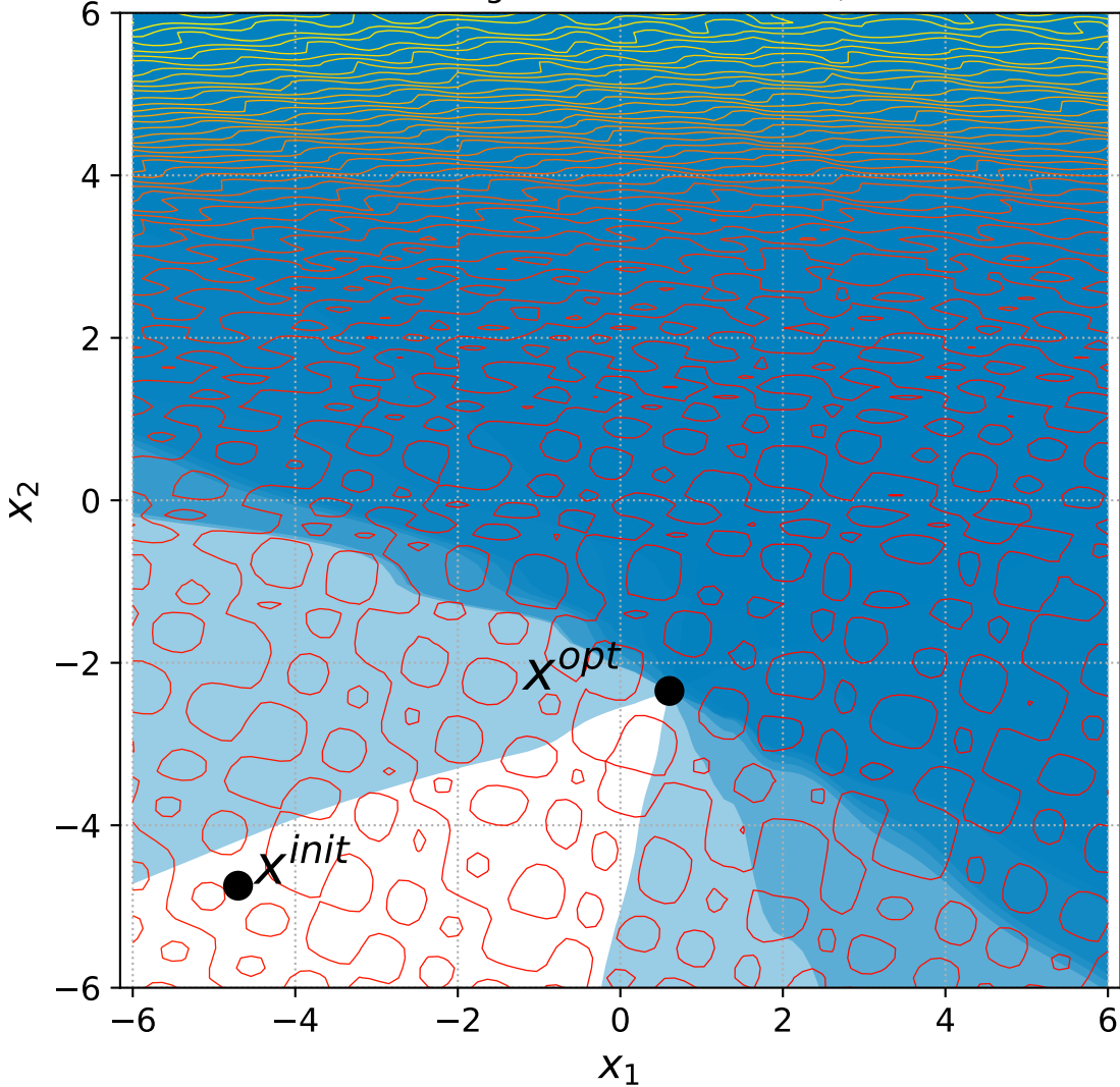
51 Rotated Rastrigin with 6 constraints, instance=3
