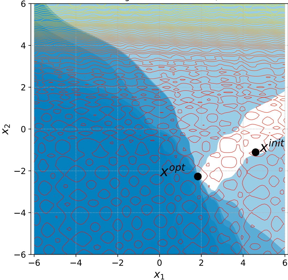
51 Rotated Rastrigin with 6 constraints, instance=2
