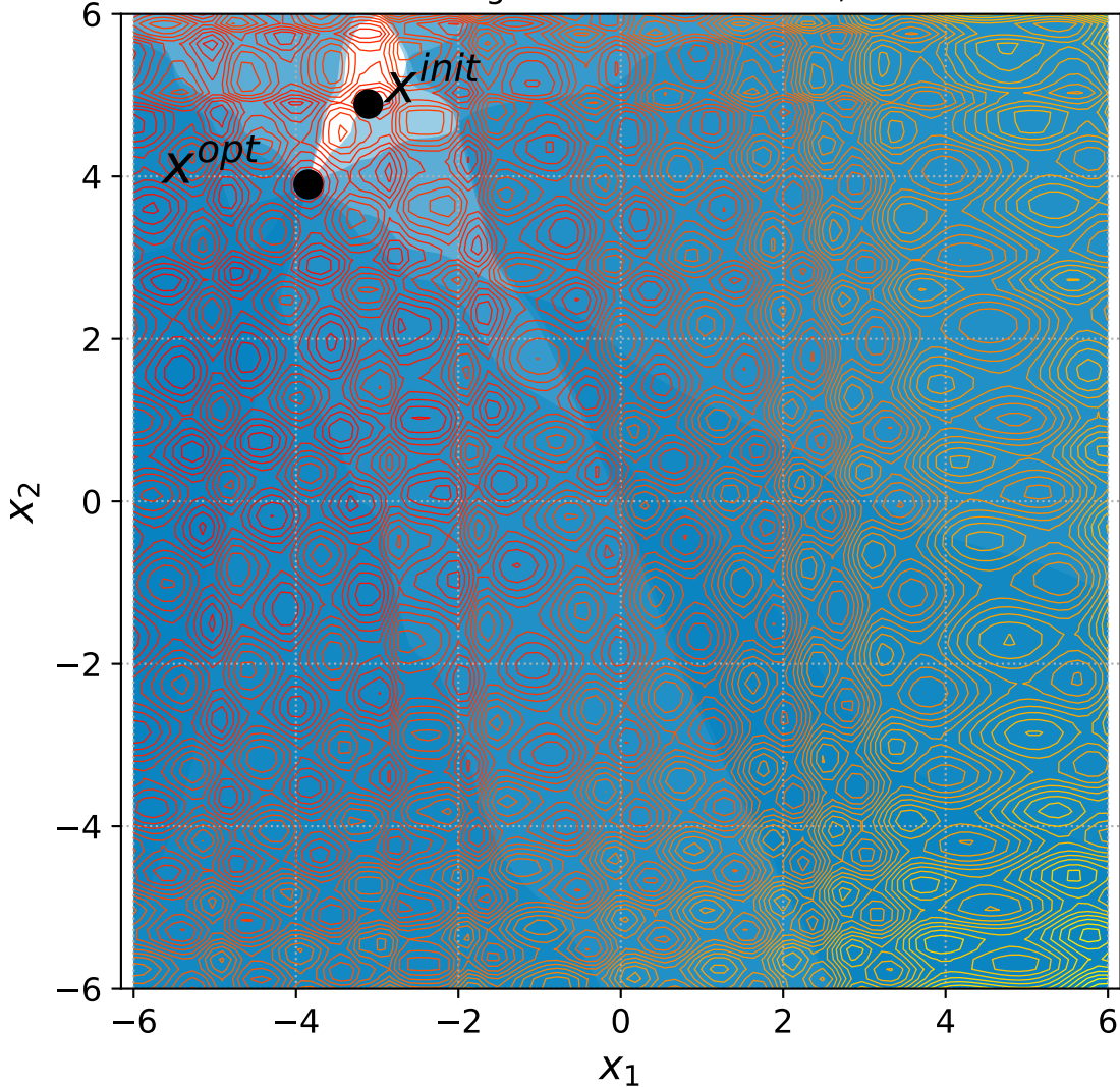
51 Rotated Rastrigin with 6 constraints, instance=1
