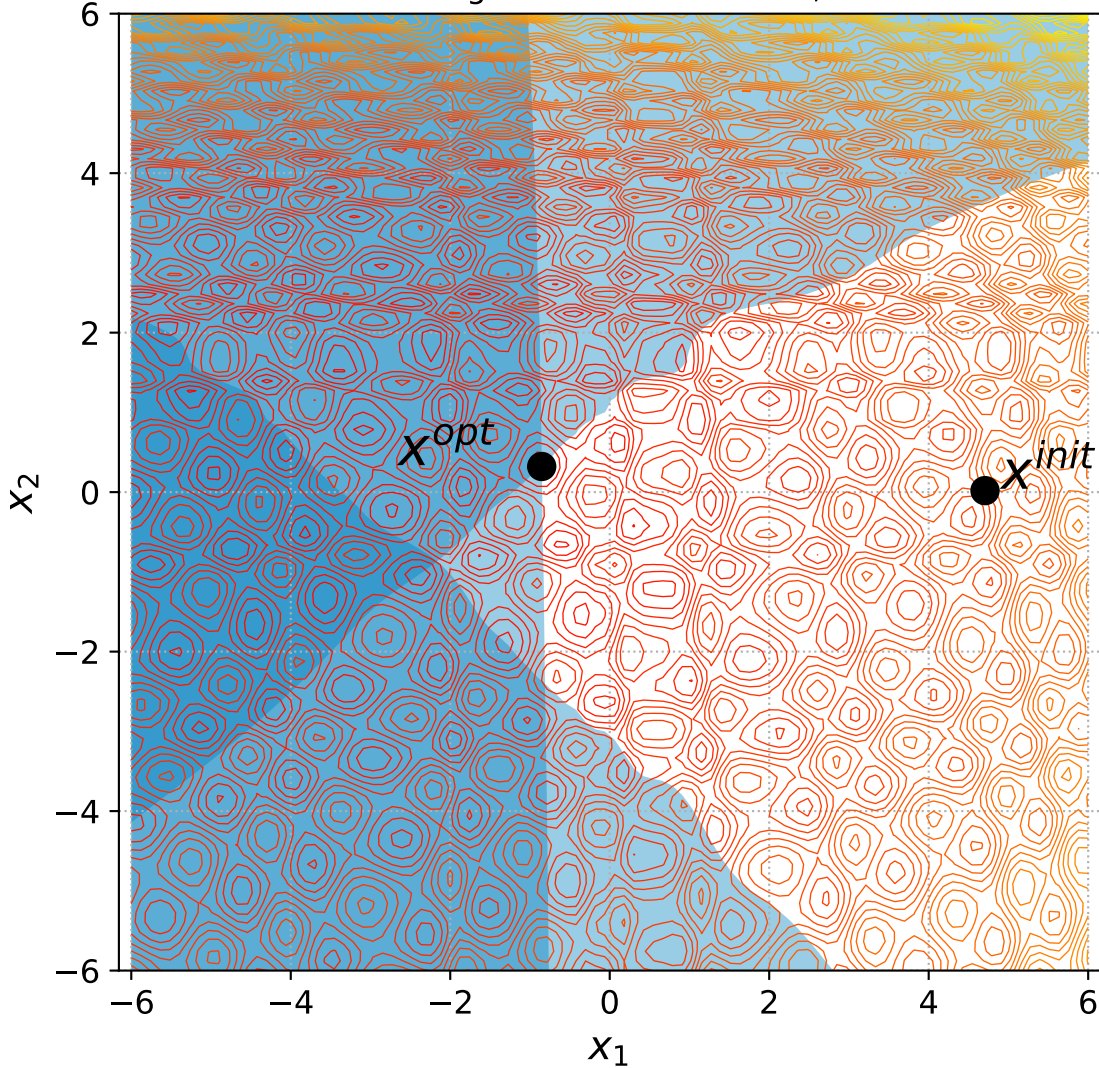
50 Rotated Rastrigin with 2 constraints, instance=15
