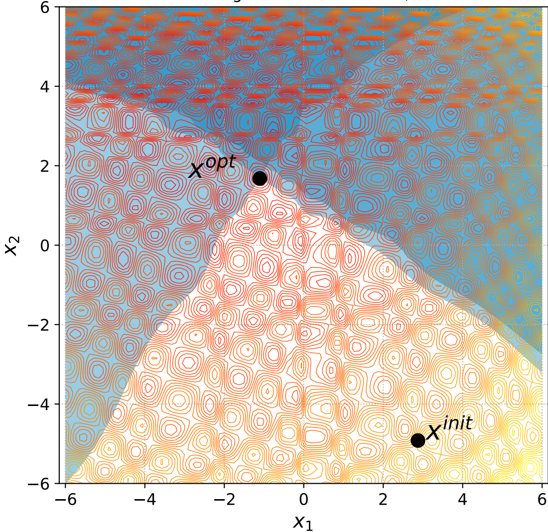
50 Rotated Rastrigin with 2 constraints, instance=14
