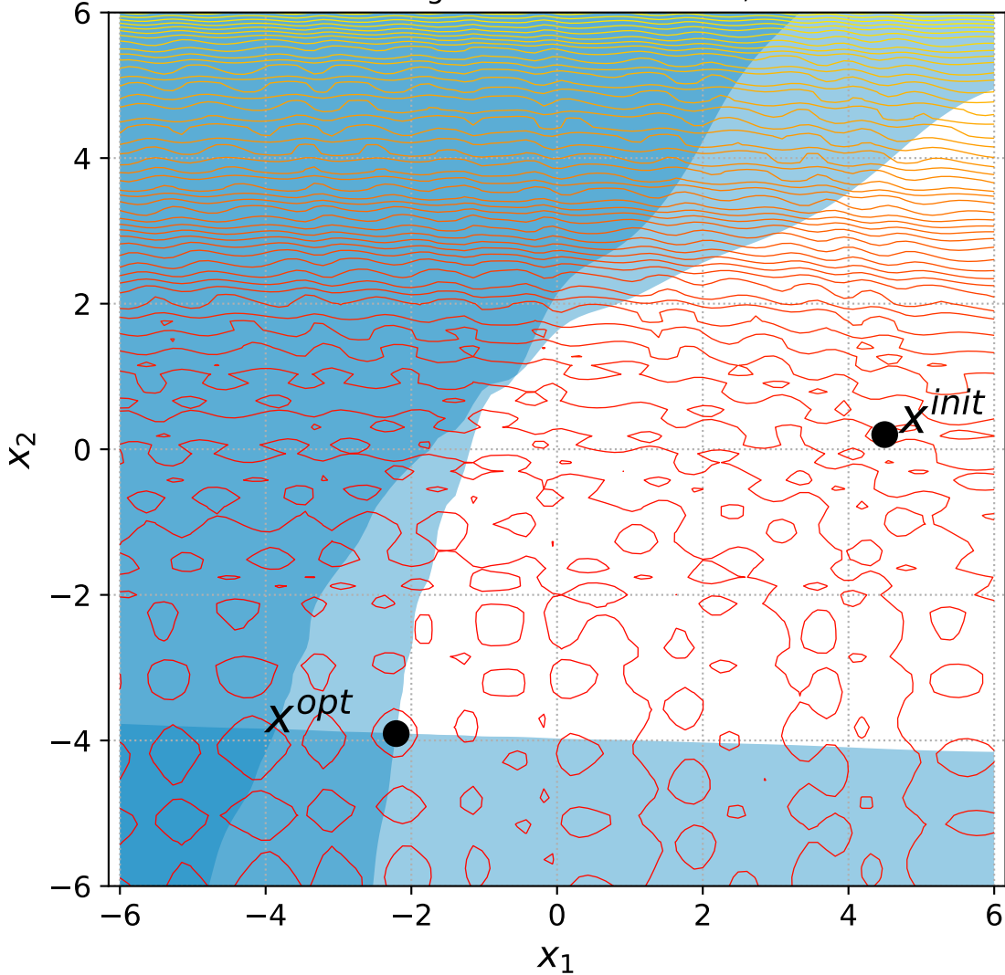
50 Rotated Rastrigin with 2 constraints, instance=13
