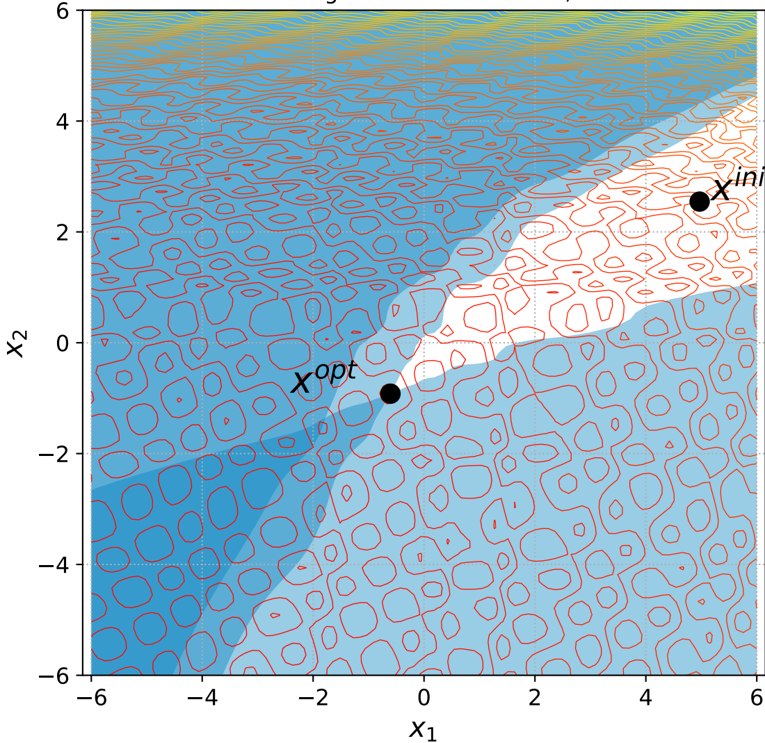
50 Rotated Rastrigin with 2 constraints, instance=12
