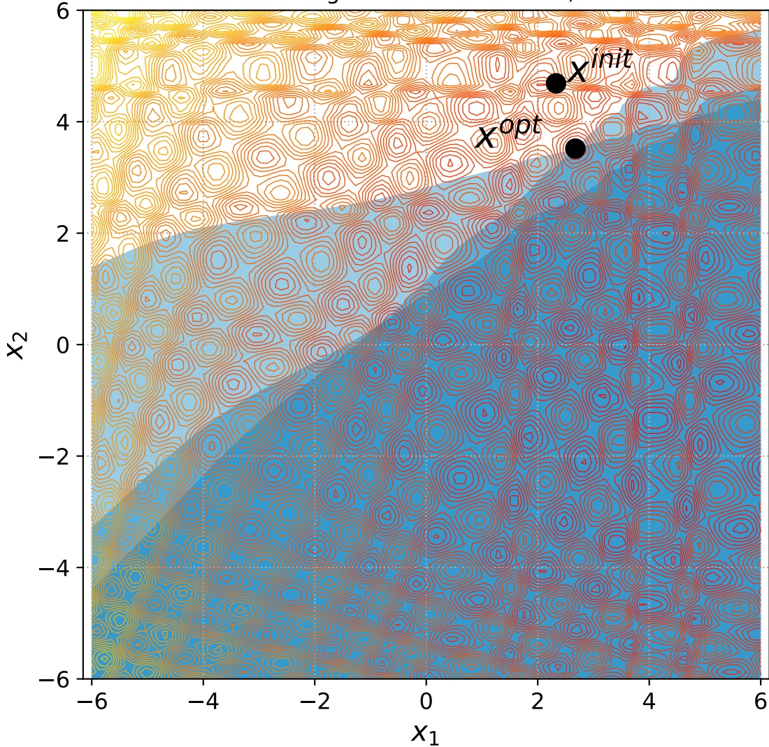
50 Rotated Rastrigin with 2 constraints, instance=10
