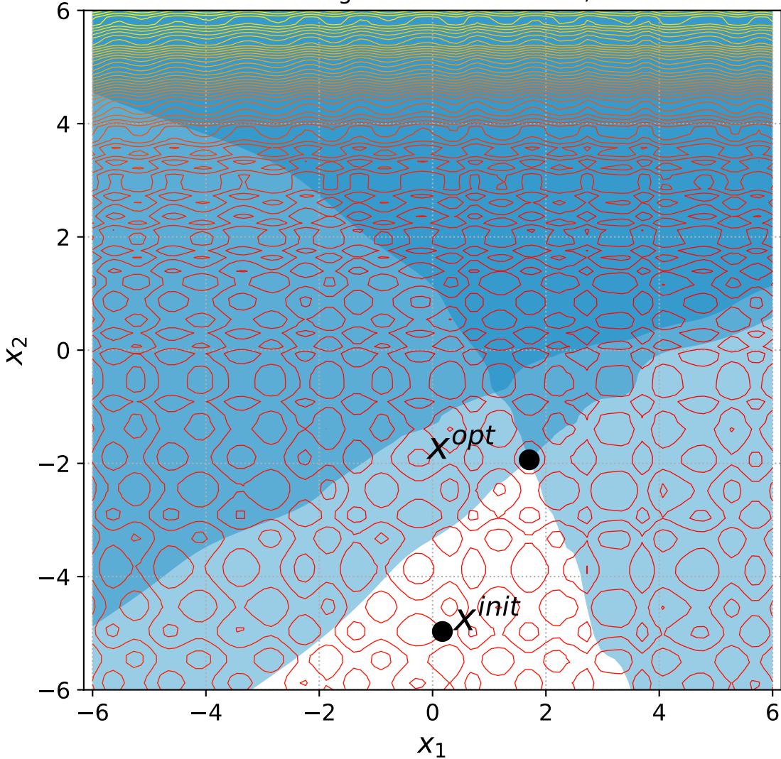
50 Rotated Rastrigin with 2 constraints, instance=7
