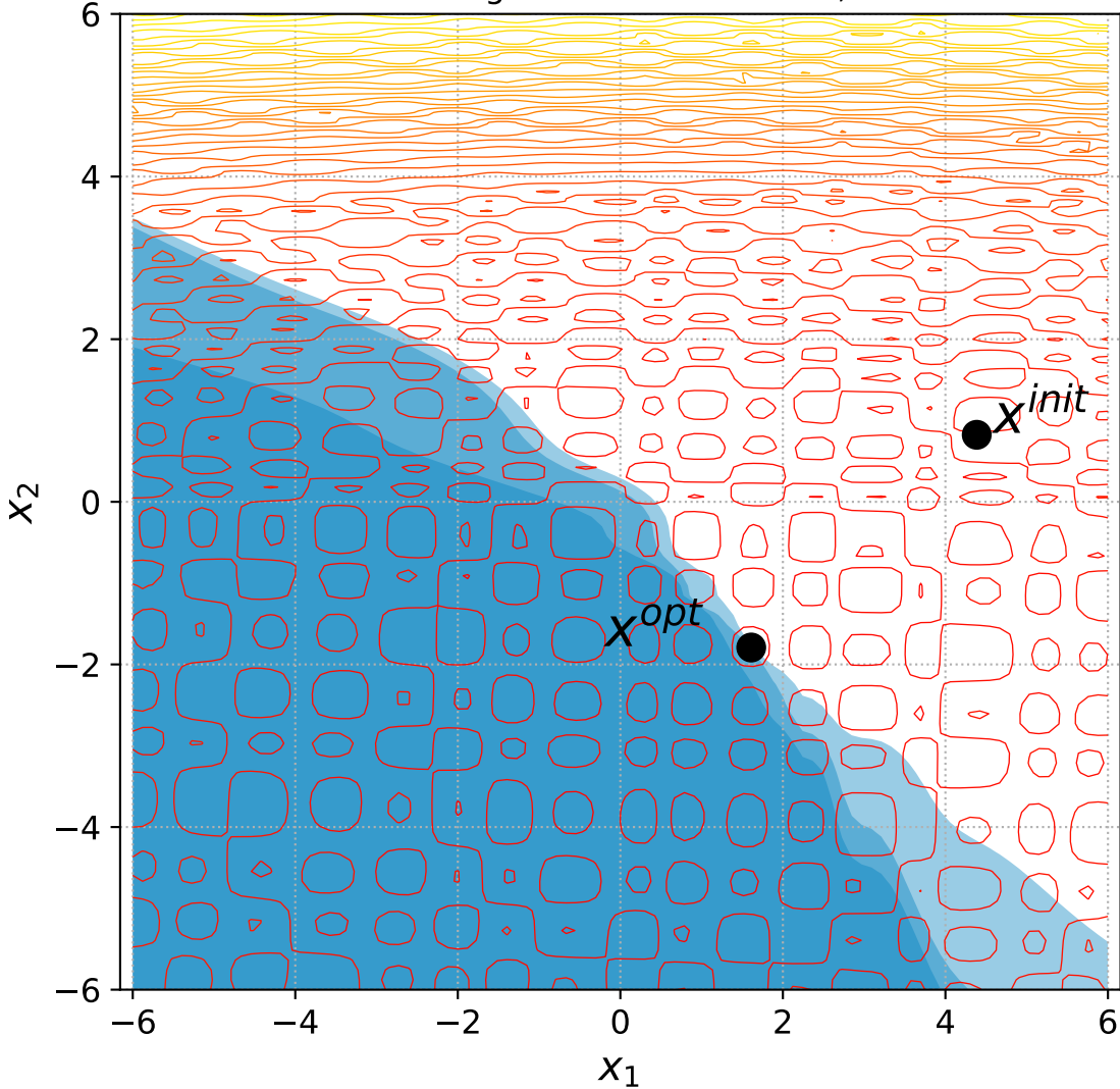
50 Rotated Rastrigin with 2 constraints, instance=6
