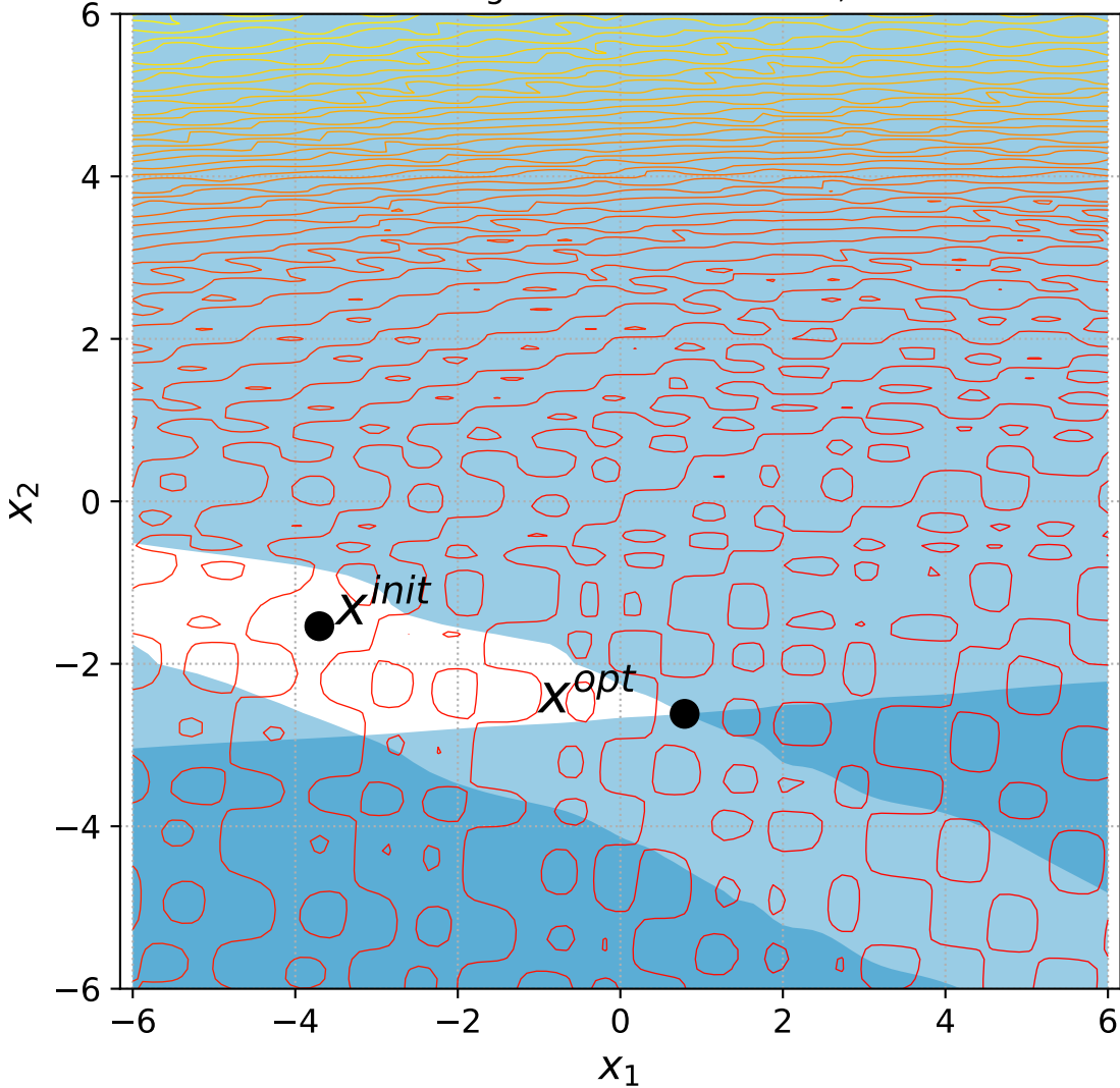
50 Rotated Rastrigin with 2 constraints, instance=5
