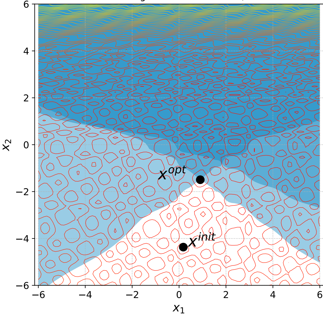
50 Rotated Rastrigin with 2 constraints, instance=4
