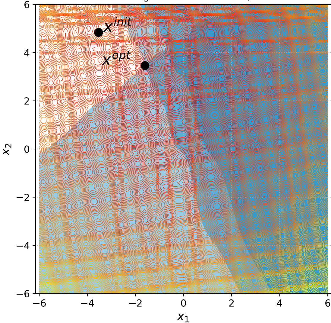
50 Rotated Rastrigin with 2 constraints, instance=2
